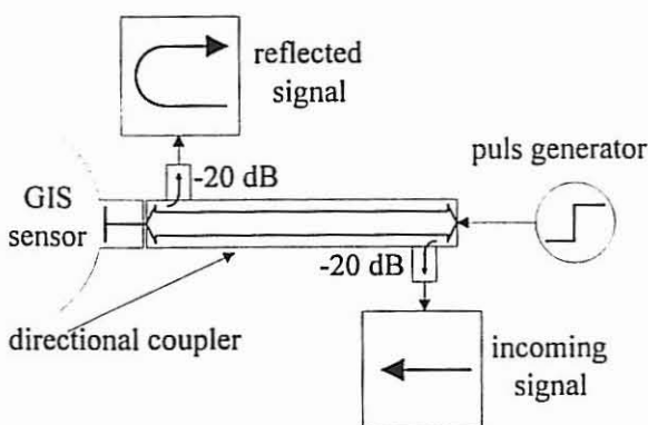
Fig. 7: Measurement setup for the determination of the pulse reflection at the sensor
