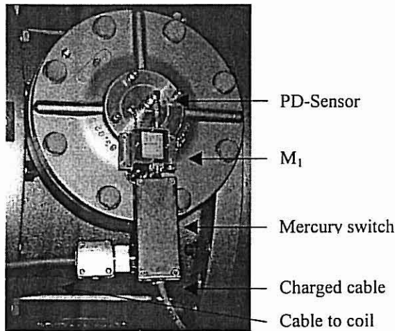
Fig. 2: Mercury switch with matching unit connected to a PD sensor
