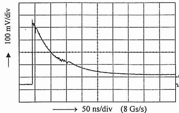
Fig. 5: Pulse shape with a charging cable of 1 meter. The very fast rise time of the realized pulse generator is a direct result of the optimized source impedance match to 50 \Omega . The mercury switch is mounted in a
