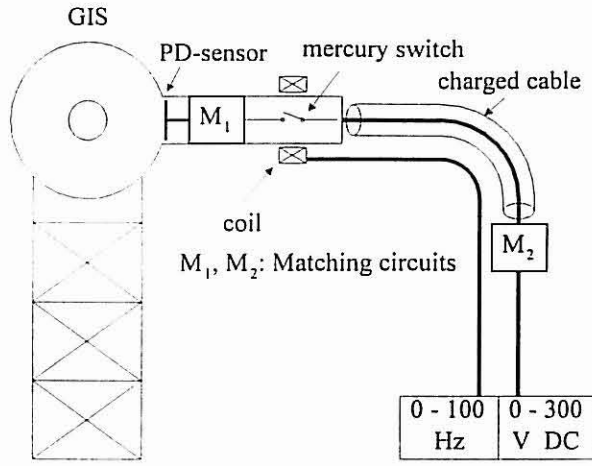
Fig. 1: Design of the pulse generator
