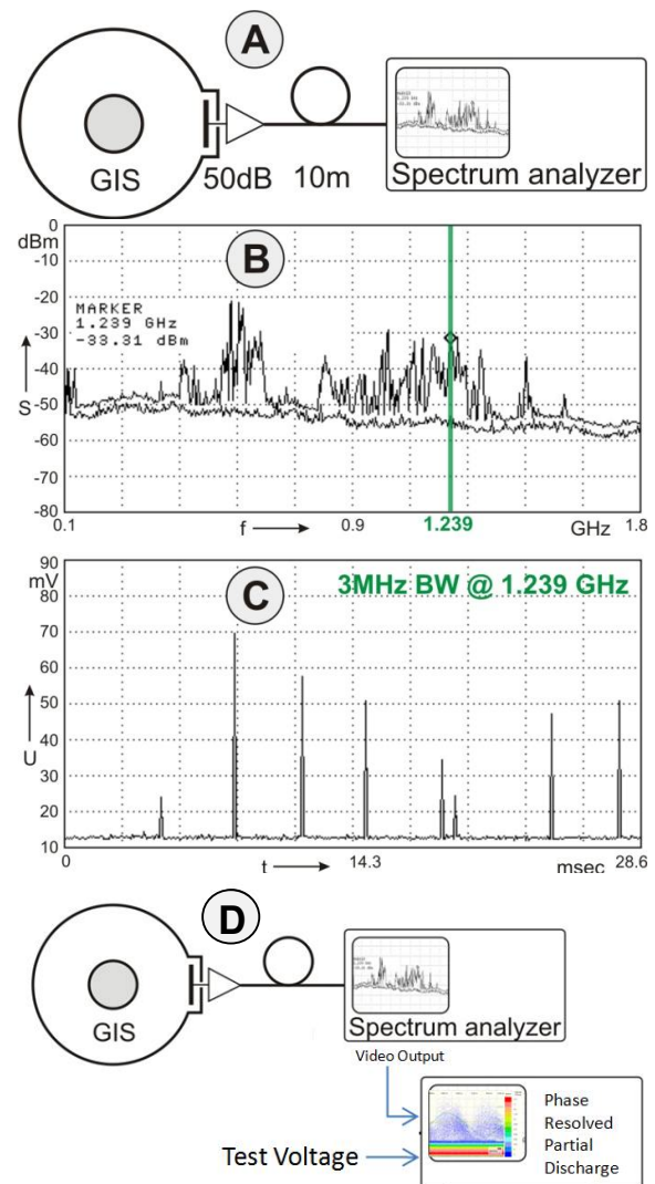
Figure 4: Example of a tuned UHF narrowband measurement with variable center frequency
